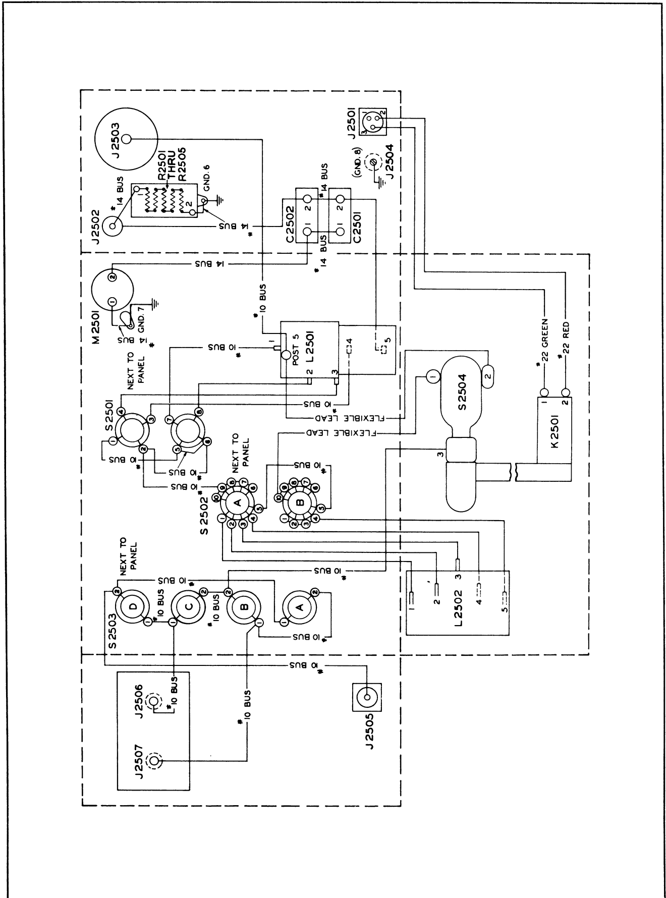
Figure 8-34. Antenna Loading Unit CU-32/ART-13A — Practical Wiring Diagram
