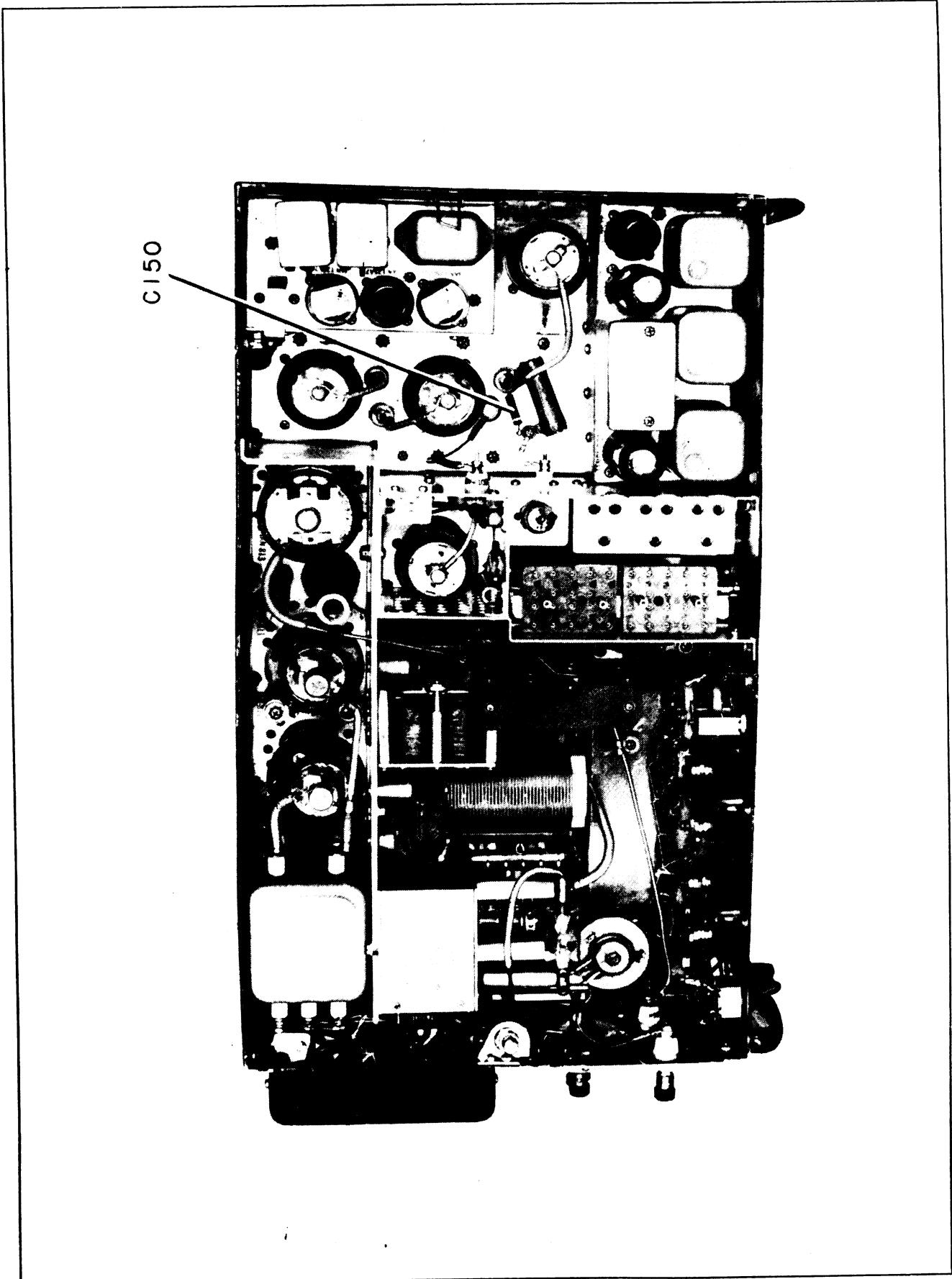
Figure 8-2A. Radio Transmitter T-412/ART-13B — Top View, Cover Removed
