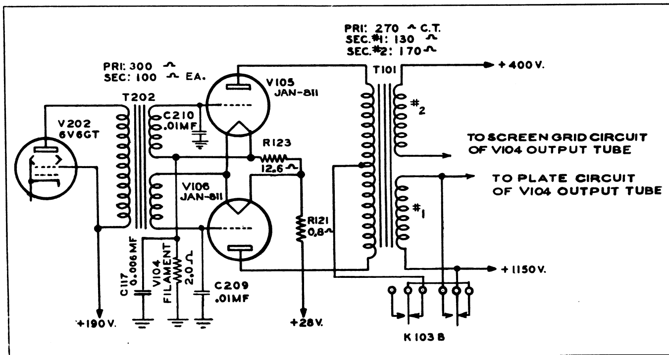
Figure 4-7. Modulator Circuit
