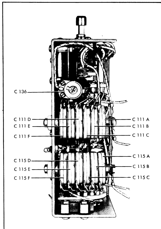
Figure 5-9. Frequency Multiplier
