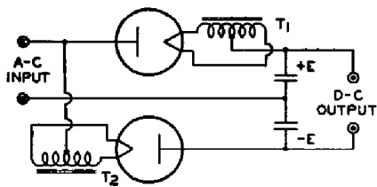
T 1 , T 2 = SEPARATE FILAMENT TRANSFORMER WINDINGS.
