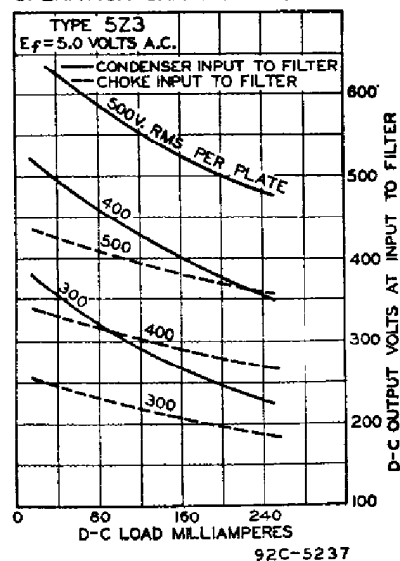
OPERATION CHARACTERISTICS
