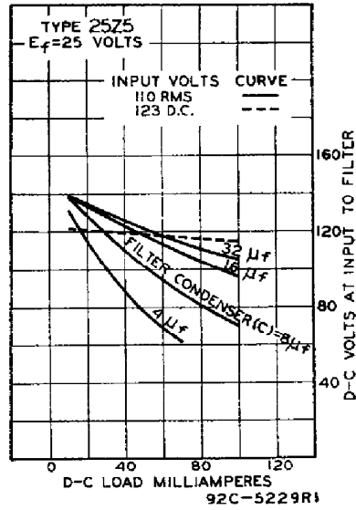
OPERATION CHARACTERISTICS HALF-WAVE RECTIFIER
