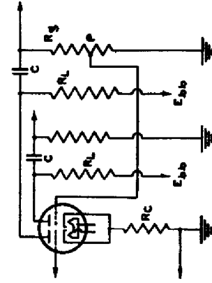
TWIN-TRIODE DIAGRAM WITH LEGEND
