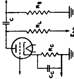
TRIODE DIAGRAM WITH LEGEND
