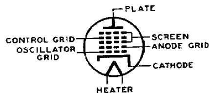
PENTAGRID CONVERTER
