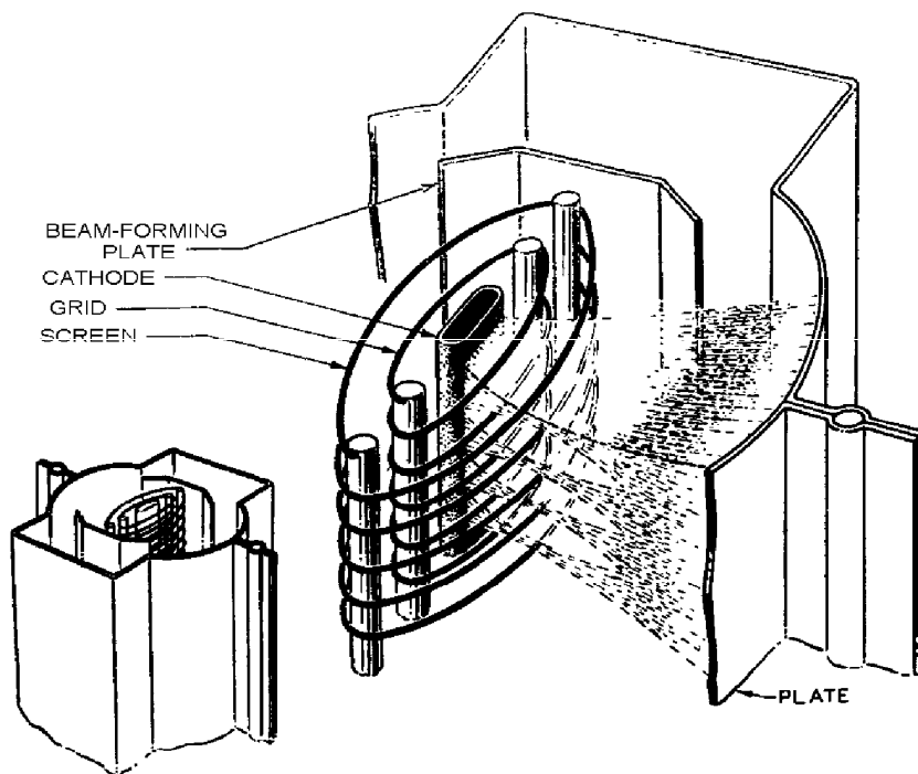
INTERNAL STRUCTURE OF BEAM POWER TUBE
