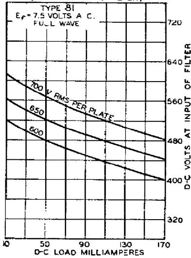
OUTPUT CHARACTERISTICS (CHOKE INPUT TO FILTER)
