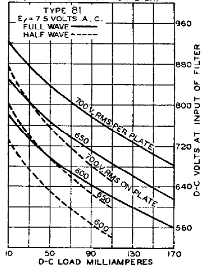
OUTPUT CHARACTERISTICS (CONDENSER INPUT TO FILTER)
