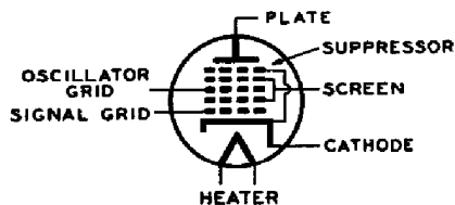
PENTAGRID MIXER
