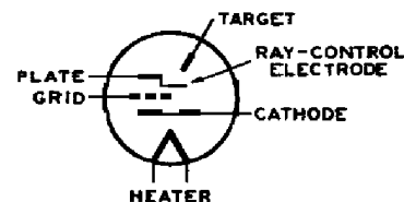
ELECTRON-RAY TUBE
