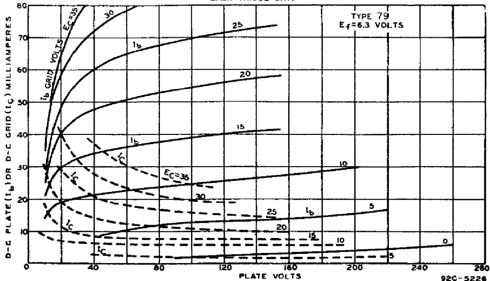
AVERAGE PLATE CHARACTERISTICS EACH TRIODE UNIT
