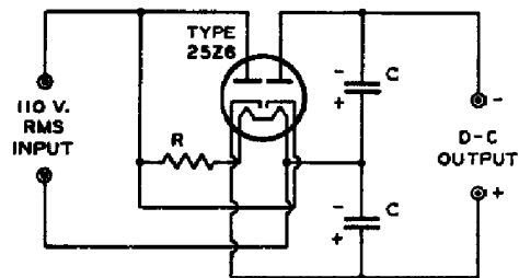
VOLTAGE-DOUBLER CIRCUIT
