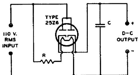
HALF-WAVE RECTIFIER CIRCUIT
