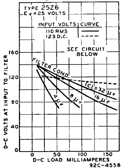
OPERATION CHARACTERISTICS HALF-WAVE RECTIFIER
