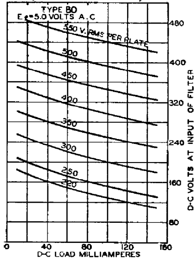
OUTPUT CHARACTERISTICS (CHOKE INPUT TO FILTER)
