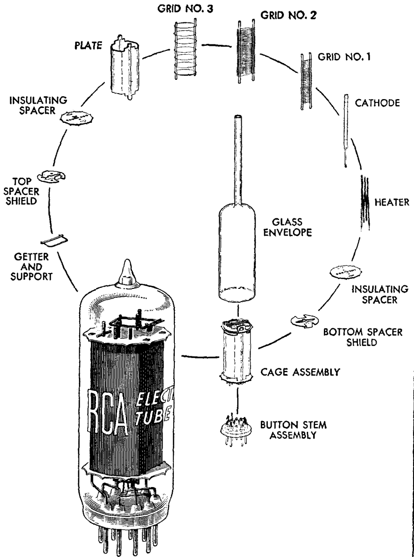
Parts of a Miniature Pentode
