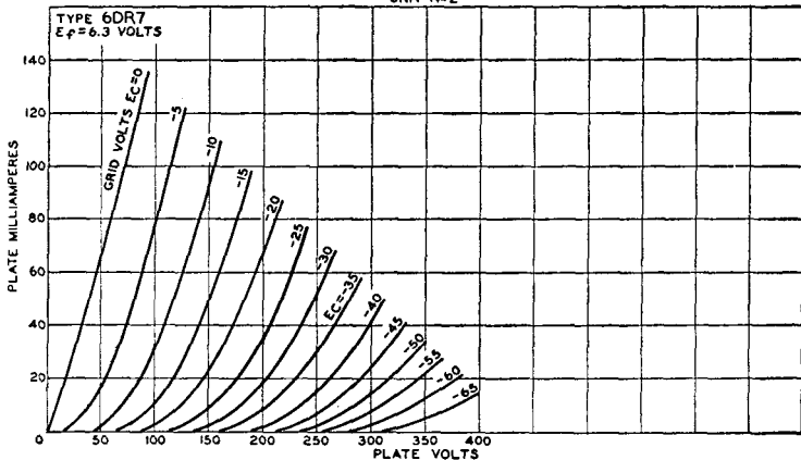
AVERAGE PLATE CHARACTERISTICS UNIT No. 2
