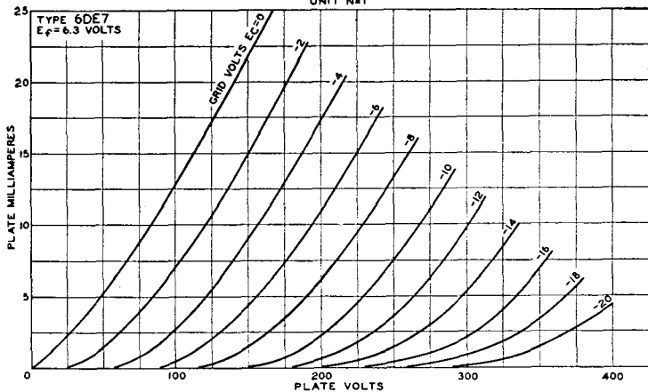
AVERAGE PLATE CHARACTERISTICS UNIT NR1
