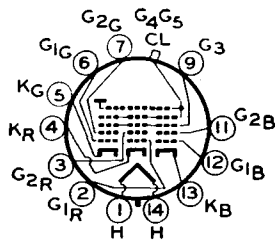
14W ULTOR = G_4 + G_5 + CL FOCUSING ELECTRODE = G_3
