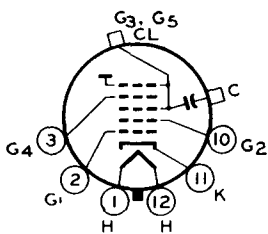
12AB ULTOR = G_3 + G_5 + CL FOCUSING ELECTRODE = G_4
