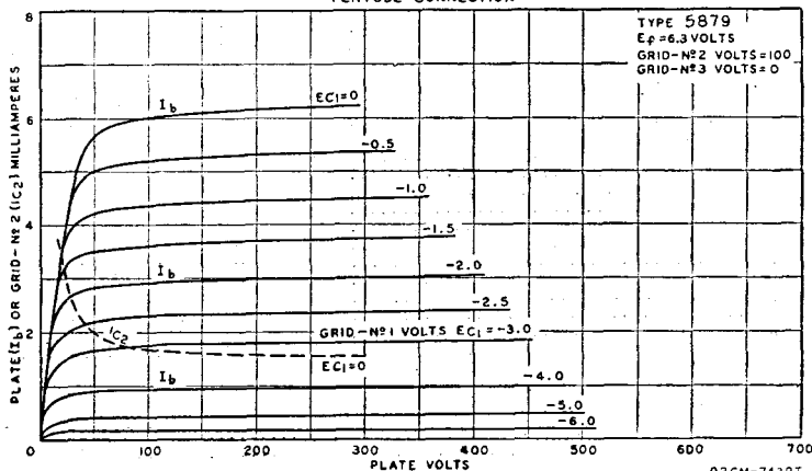
AVERAGE CHARACTERISTICS PENTODE CONNECTION
