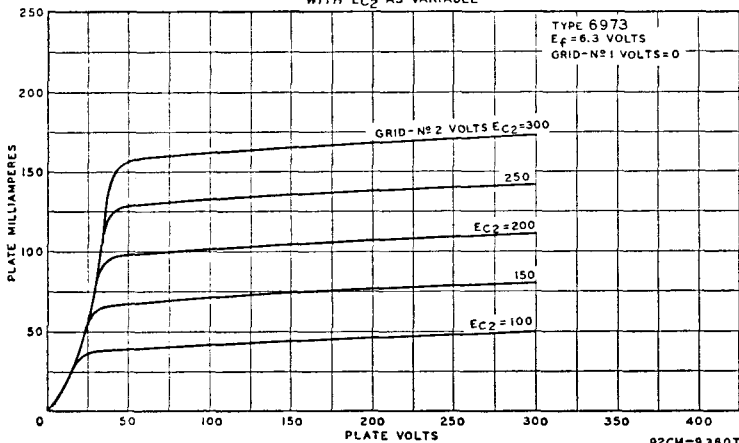
AVERAGE CHARACTERISTICS WITH E_{C2} AS VARIABLE
