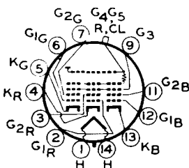
14AH ULTOR = G_4 + G_5 + CL + R FOCUSING ELECTRODE = G_3
