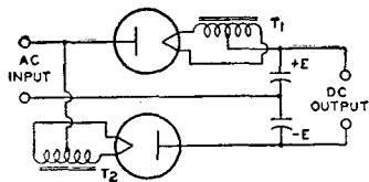
T 1 , T 2 = SEPARATE FILAMENT TRANSFORMER WINDINGS
