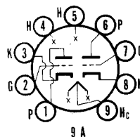
SYLVANIA TYPE 12BH7A MEDIUM-MU DUOTRIODE
