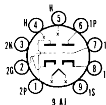
SYLVANIA TYPE 5BK7A MEDIUM-MU DUO TRIODE
