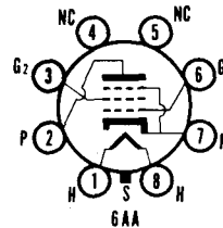
SYLVANIA TYPE 50A5 BEAM POWER AMPLIFIER
