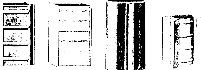
25 Watt Carbonized Nickel Plate RK-11 RK-12 40 Watt Molybdenum Plate RK-18 RK-31 60 Watt Graphite Plate RK-51 RK-52 100 Watt Tantalum Plate RK-36 RK-38
