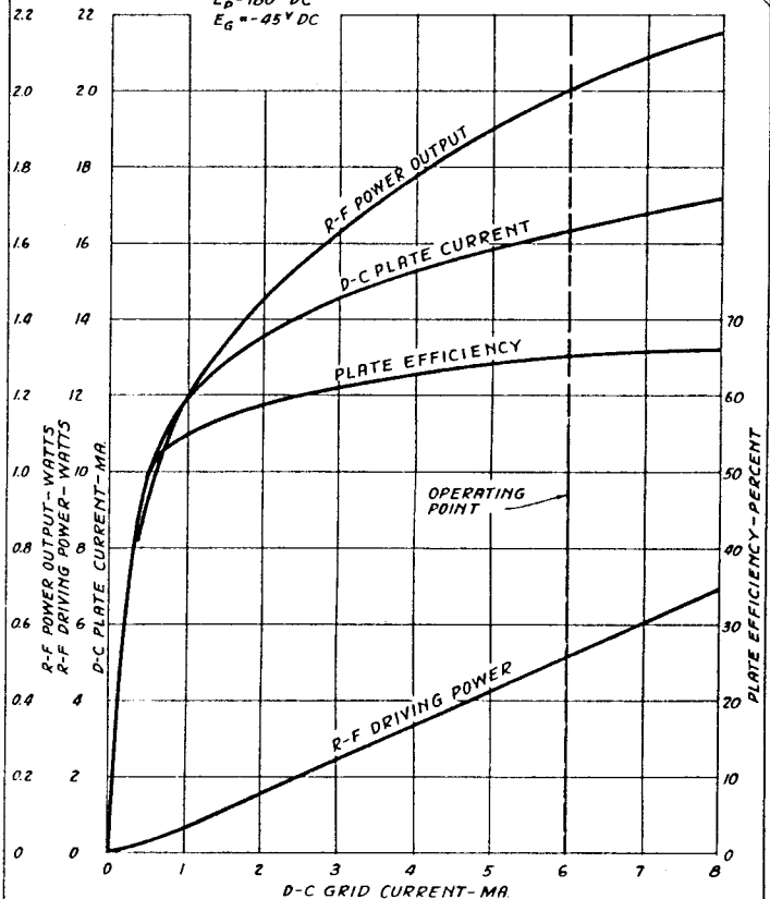
AVERAGE CHARACTERISTICS R-F POWER AMPLIFIER—CLASS C E_g = 2.0\text{V DC} E_p = 180\text{V DC} E_g = -45\text{V DC}
