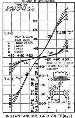
DYNAMIC TRANSFER CHARACTERISTICS
