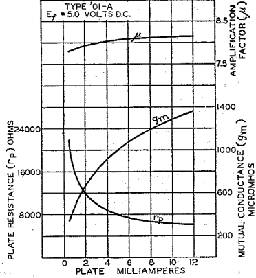
AVERAGE PLATE CHARACTERISTICS
