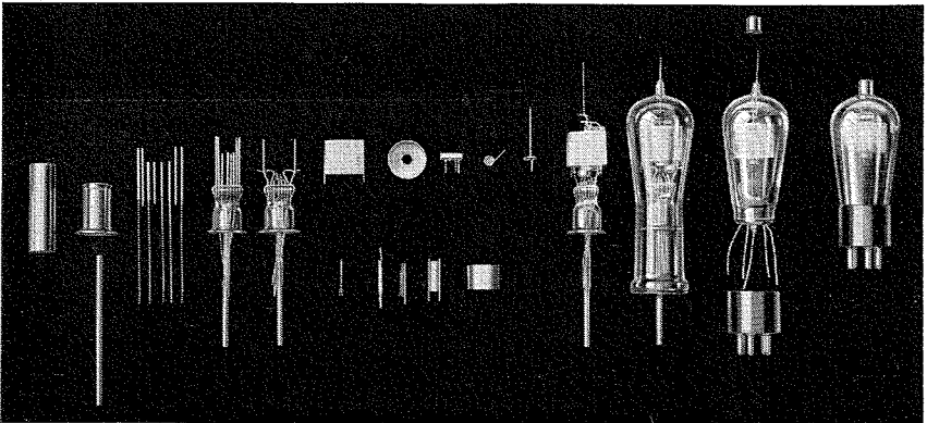
Parts Assembly of the '24-A
