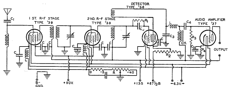
DIAGRAMMATIC SHORTWAVE RECEIVER 6.3-VOLT HEATER TYPE TUBES
