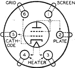
Tube Symbol and Top View of Socket Connections
