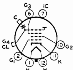
12C ULTOR = G_4 + CL FOCUSING ELECTRODE = G_3
