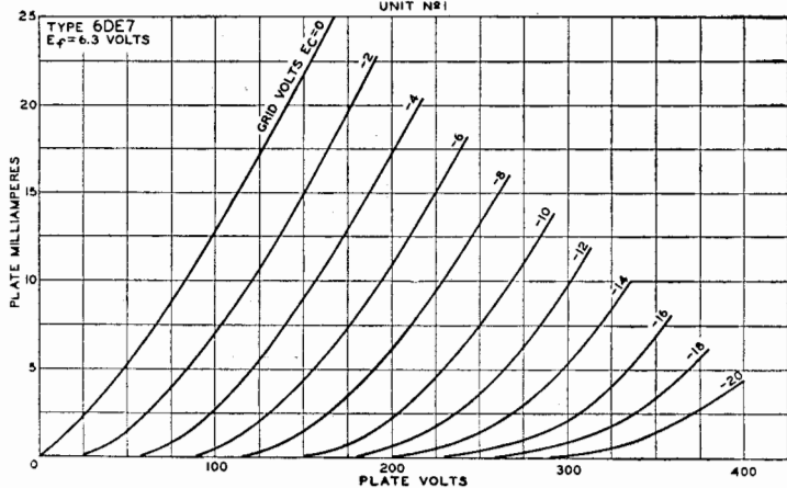
AVERAGE PLATE CHARACTERISTICS UNIT NR1
