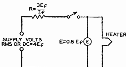
E_f = RATED HEATER VOLTAGE I_f = RATED HEATER CURRENT
