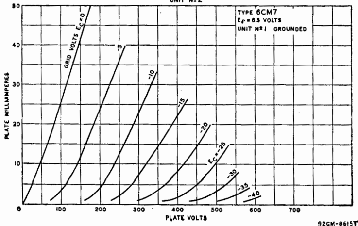
AVERAGE CHARACTERISTICS UNIT #2
