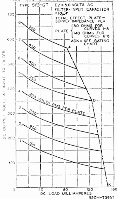
OPERATION CHARACTERISTICS FULL-WAVE CIRCUIT, CAPACITOR INPUT TO FILTER
