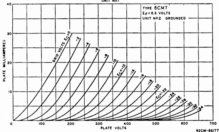
AVERAGE CHARACTERISTICS UNIT #1
