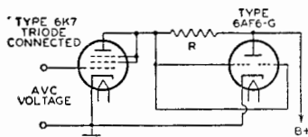
R: TYPICAL VALUE IS 0.5 MEGOHM Fig. 66
