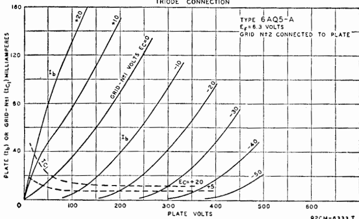
AVERAGE CHARACTERISTICS TRIODE CONNECTION
