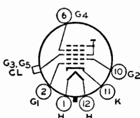
12M ULTOR = G_3 + G_5 + CL FOCUSING ELECTRODE = G_4
