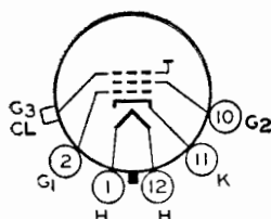
12D ULTOR = G_3 + CL
