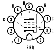
SYLVANIA TYPE 6BK5 BEAM POWER AMPLIFIER
