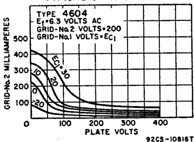
TYPICAL CHARACTERISTICS
